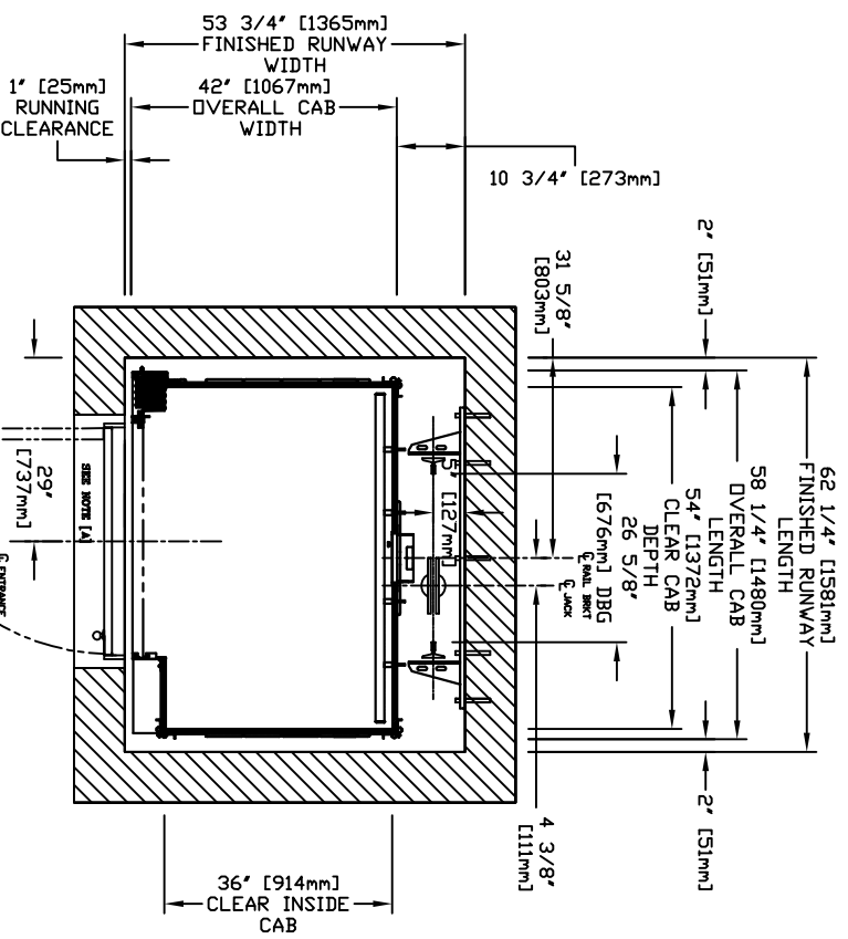
PLAN VIEW - INFINITY Model 3654 TYPE 5
