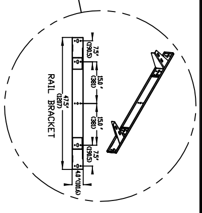
RAIL BRACKET
