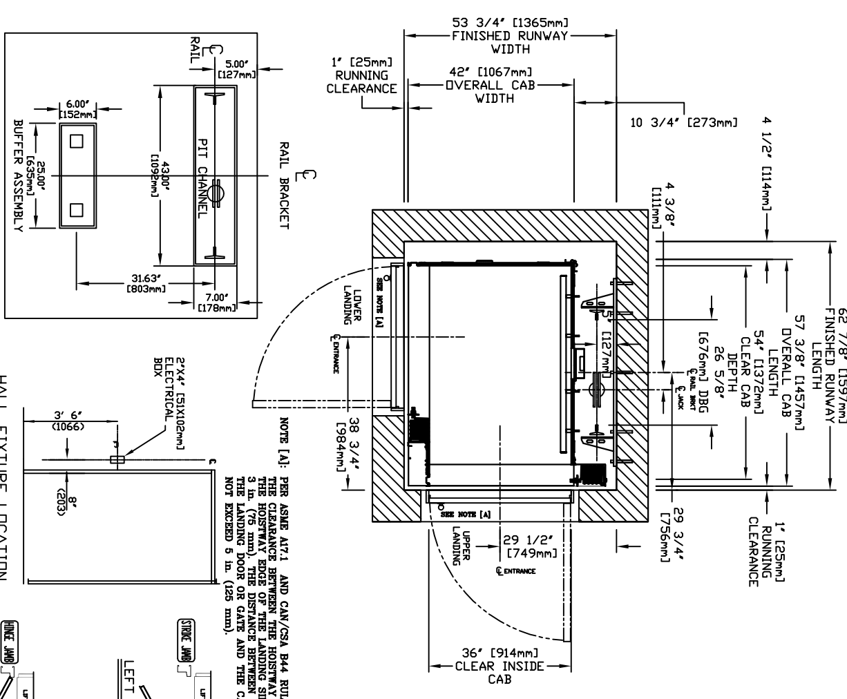
PLAN VIEW - INFINITY Model 3654 TYPE 3
