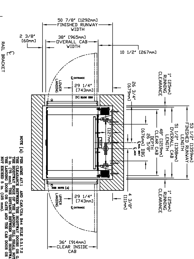
PLAN VIEW - INFINITY Model 3648 TYPE 2
