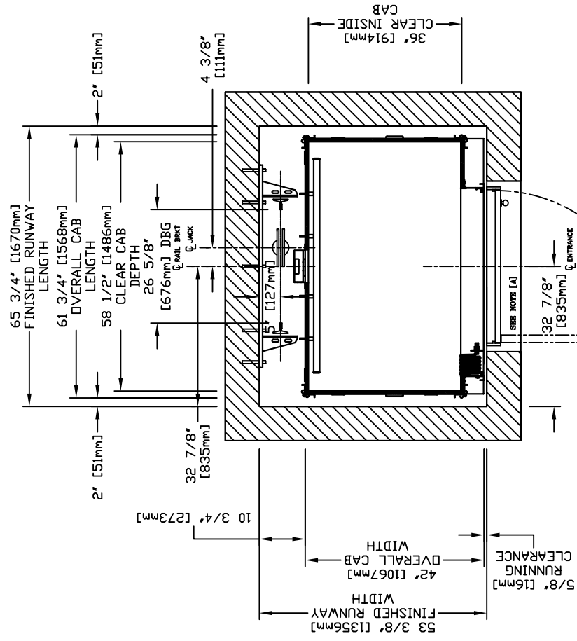
PLAN VIEW - INFINITY Model 3660 TYPE 5
