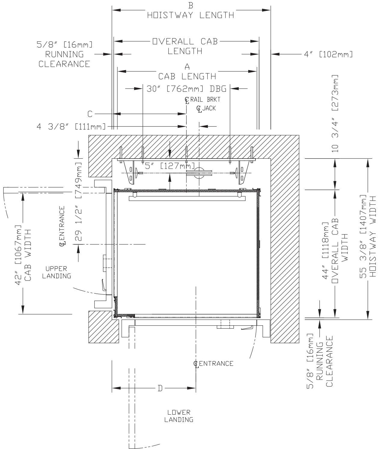
HOISTWAY DIMENSIONS
